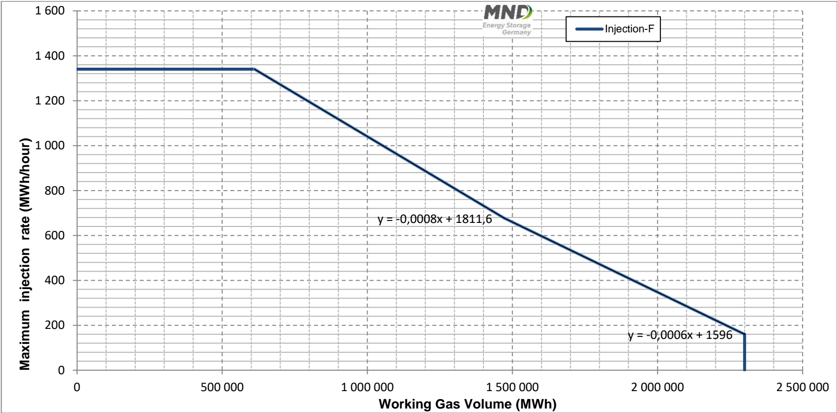
Injection curve
